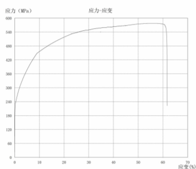
Fig.1-1 JC260806001-01 Stress-strain curve
