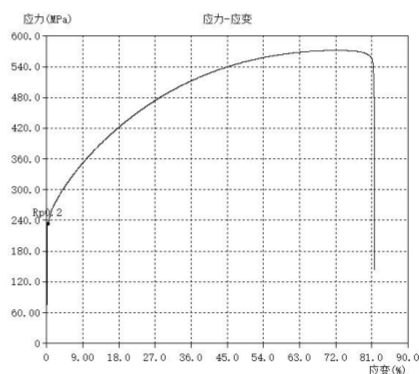
Fig.1-2 JC260806001-02 Stress-strain curve
