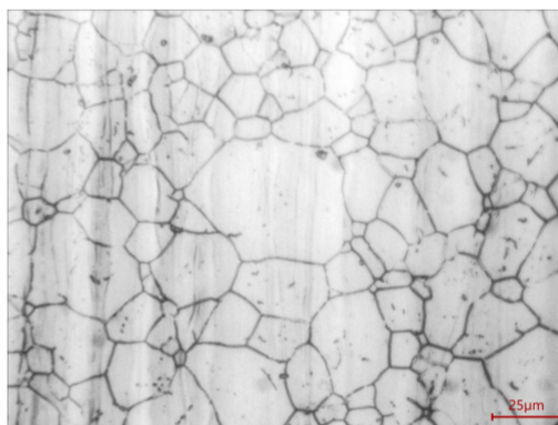
Fig.2-2 JC260806001-02 400X
